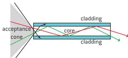
▲ Figure 6 Dispersion.
