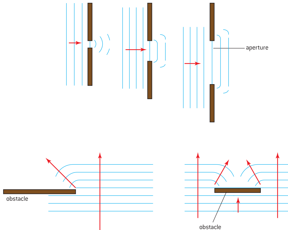
▲ Figure 5 Diffraction.
