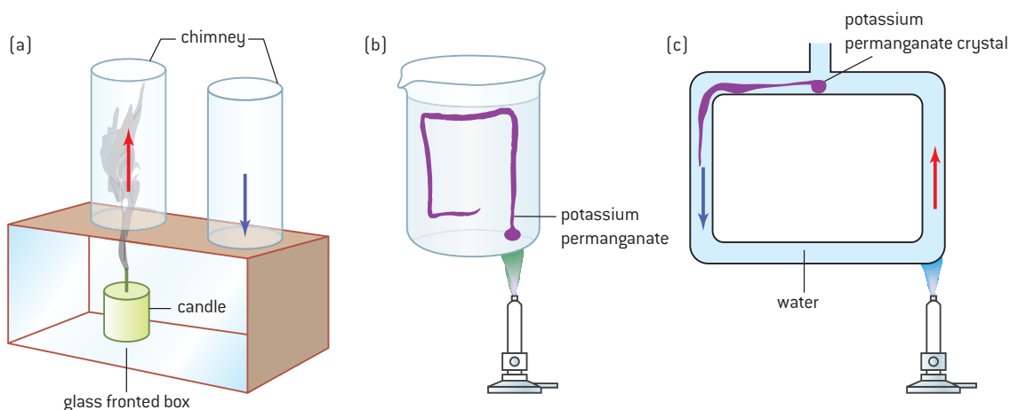
▲ Figure 3 Convection currents.
