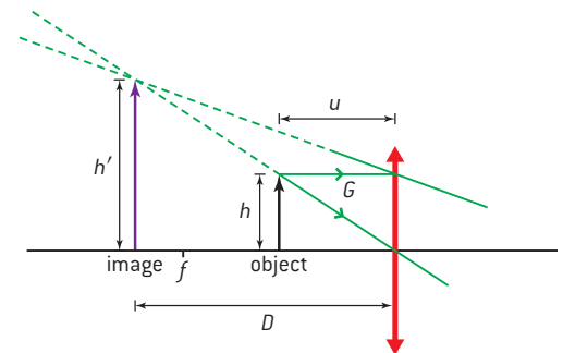
▲ Figure 17 Angular magnification for a magnifying glass.
