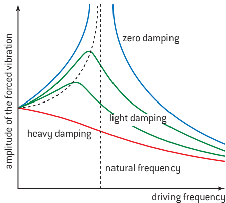
▲ Figure 4 Effect of damping on resonance.
