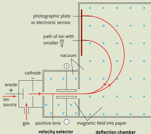
▲ Figure 18 Bainbridge mass spectrometer.
