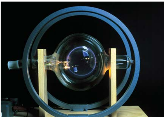
▲ Figure 14 Electrons moving in a circle demonstrated in a fine-beam tube.
