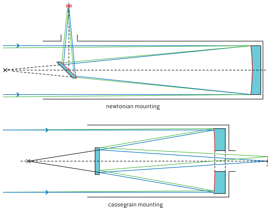
▲ Figure 8 Newtonian and cassegrain mirror systems.
