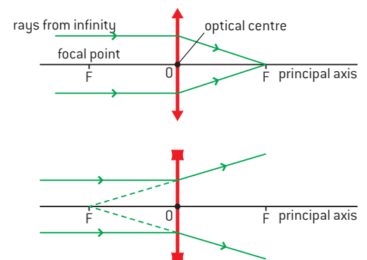
▲ Figure 10 Definitions of the parts of a lens.
