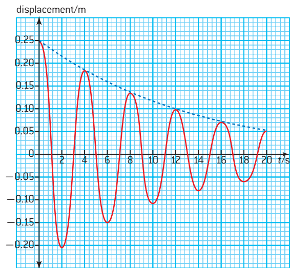
▲ Figure 1 Under-damped vibration.
