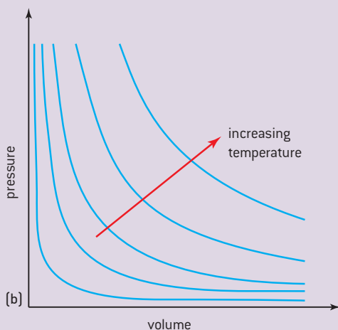
▲ Figure 2 (a) Boyle's law apparatus and (b) graph.
