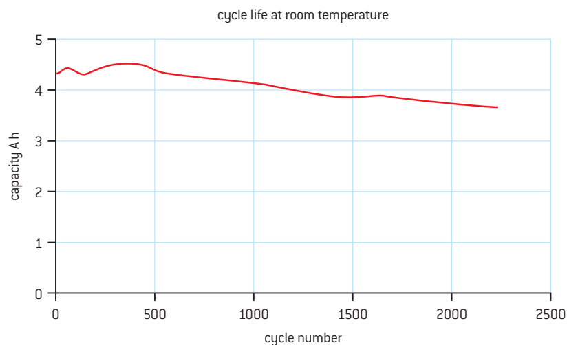
▲ Figure 4 Cycle life of a rechargeable cell.
