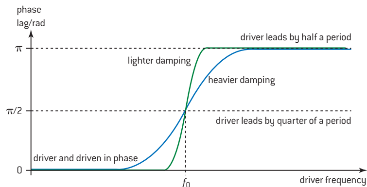
▲ Figure 6 Phase relationship for the displacement of a forced vibration.
