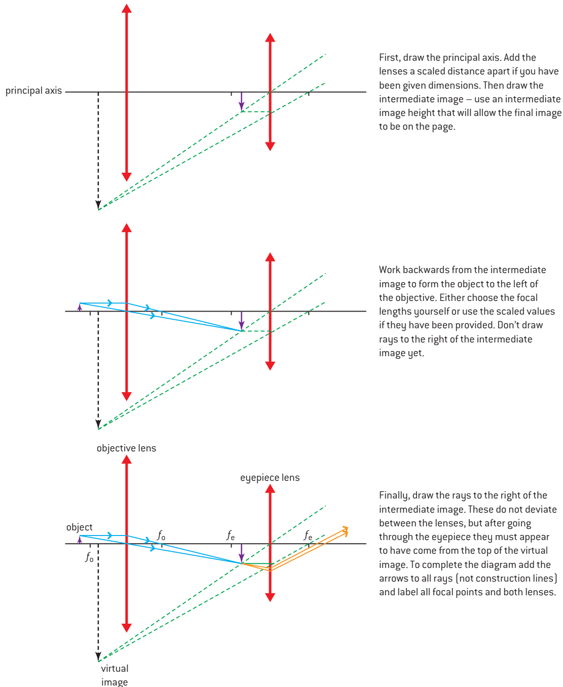
▲ Figure 3 Strategy for drawing the compound microscope diagram.
