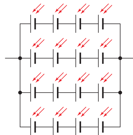
▲ Figure 14 Connecting photovoltaic cells together.
