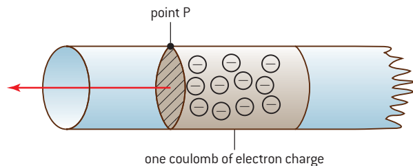
▲ Figure 16 Charge flow leading to current.
