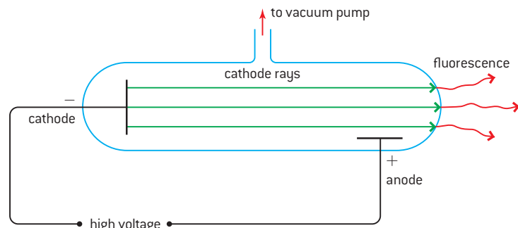
▲ Figure 1 Discharge tube.
