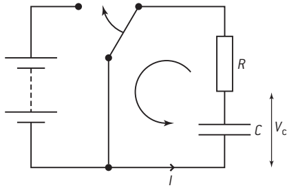
▲ Figure 8 Discharging circuit.
