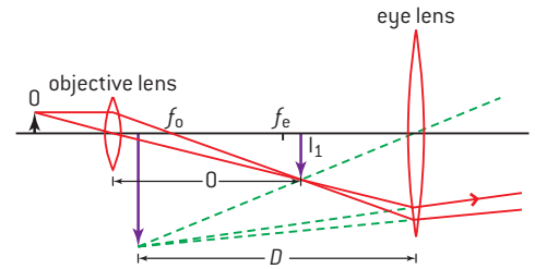
▲ Figure 1 Compound microscope.
