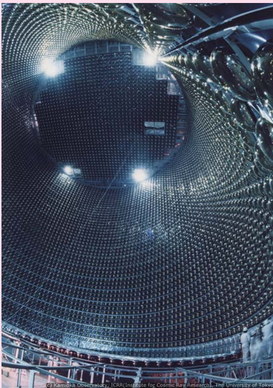
▲ Figure 8 Super-Kamiokande Neutrino Detection Experiment Mount Kamioka near Hida, Japan.
