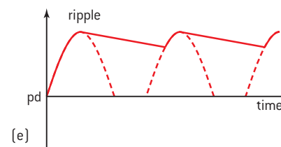
▲ Figure 10 Half-wave rectifier.
