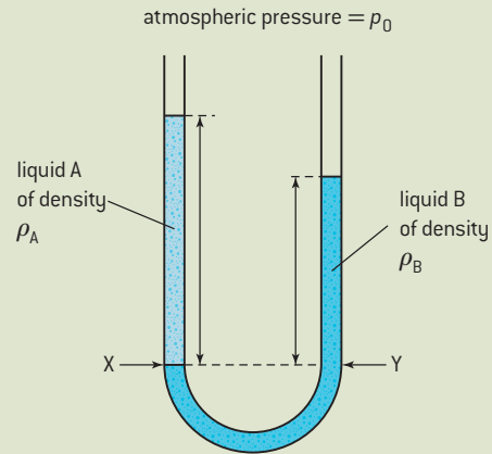
▲ Figure 3 Hydrostatic equilibrium to measure density.
