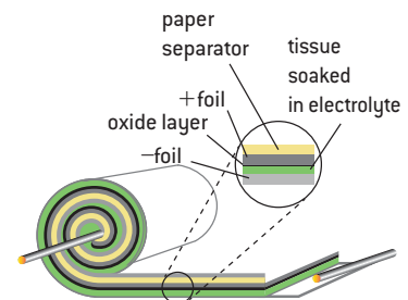
▲ Figure 5 Practical capacitors.
