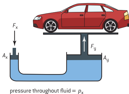
▲ Figure 4 Hydraulic jack.
