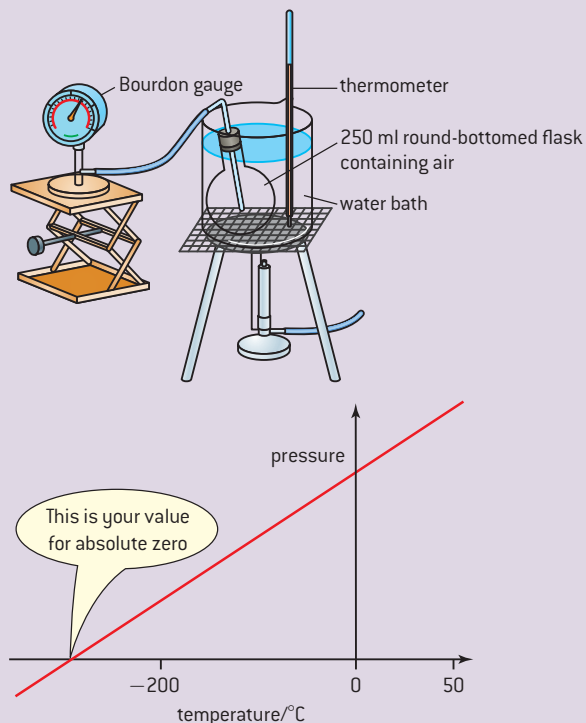
▲ Figure 4 Third gas law apparatus and graph.
