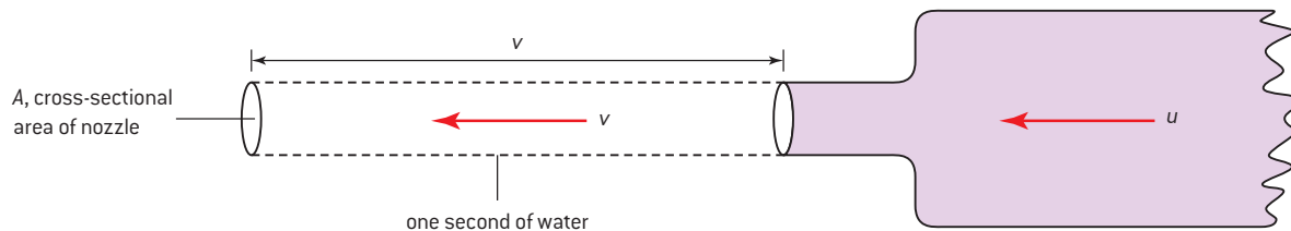
▲ Figure 9 Water leaving the hose.
