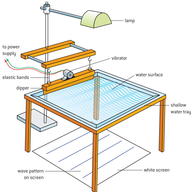
▲ Figure 1 A ripple tank.
