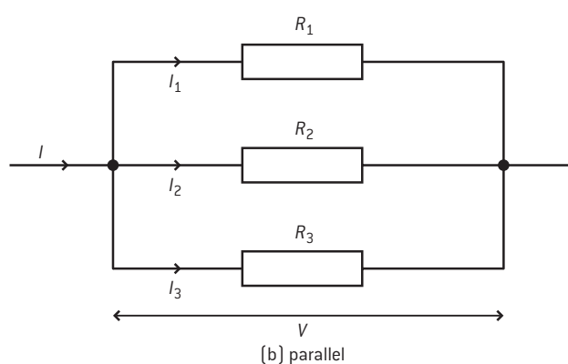
▲ Figure 11 Resistors in series and parallel.
