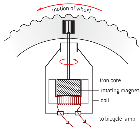
▲ Figure 2 Bicycle dynamo.
