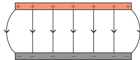
▲ Figure 2 Electric field line pattern for parallel plates.
