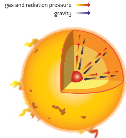
▲ Figure 4 Hydrostatic equilibrium.
