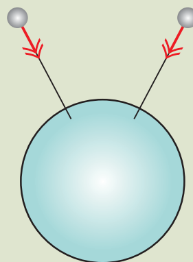
▲ Figure 3 Tidal effects.
