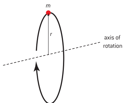
▲ Figure 4 Moment of inertia of a point mass.
