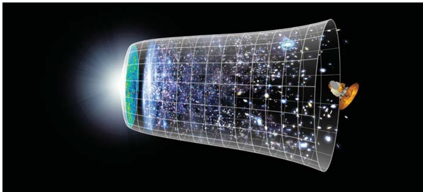
▲ Figure 5 Evolution of the accelerating universe.
