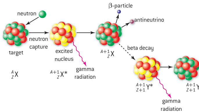
▲ Figure 4 Neutron capture.
