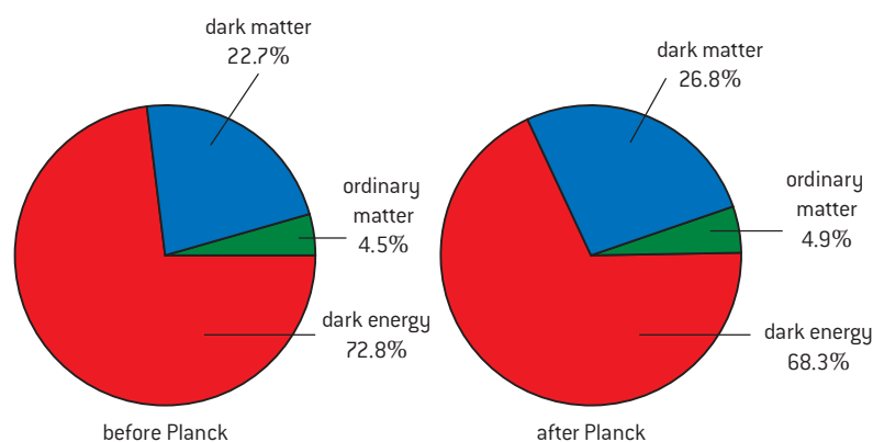
▲ Figure 9 The mass/energy recipe for the universe.
