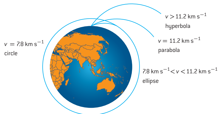
▲ Figure 12 Orbital shapes of satellites.
