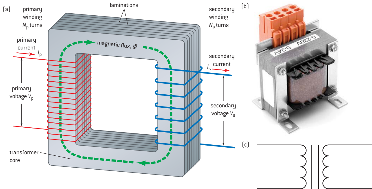
▲ Figure 6 Transformers in theory and practice.
