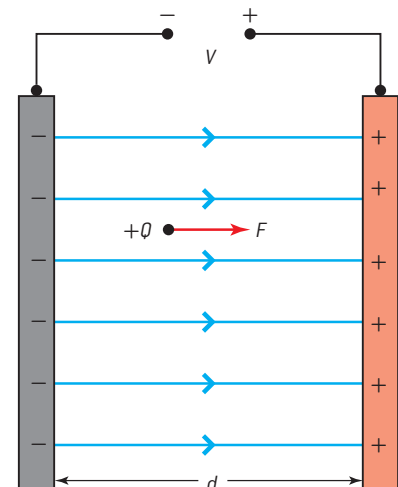
▲ Figure 2 Field strength between parallel plates.
