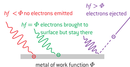
▲ Figure 3 Photoelectric emission and the work function.
