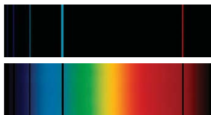
▲ Figure 4 Emission and absorption spectra for hydrogen.
