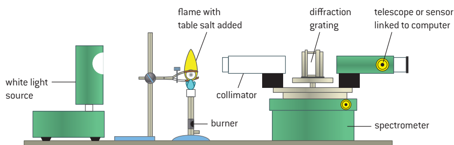
▲ Figure 5 Demonstration of sodium absorption spectra.
