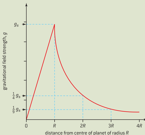
▲ Figure 6 Gravitational field strength inside and outside the Earth.
