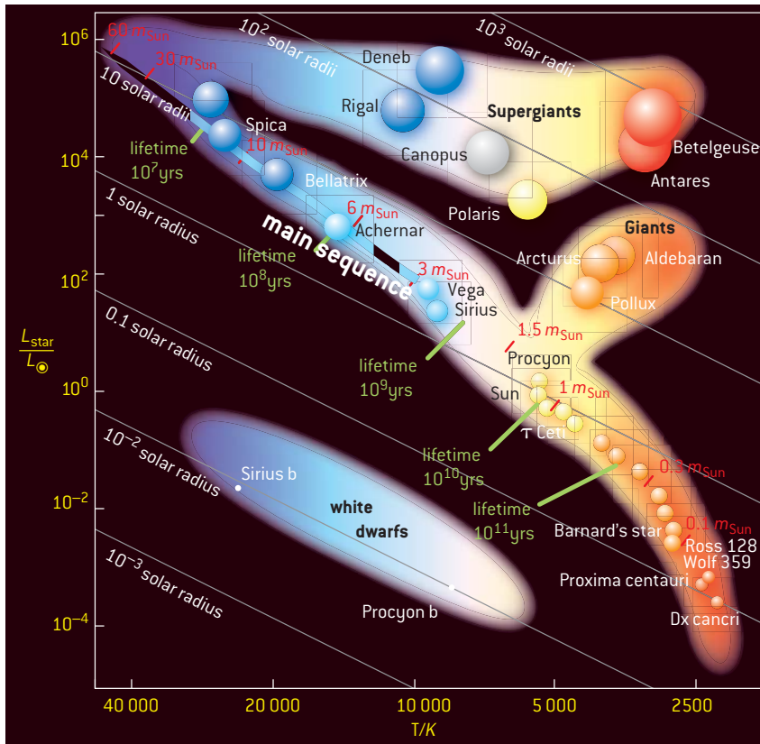
▲ Figure 6 HR diagram.
