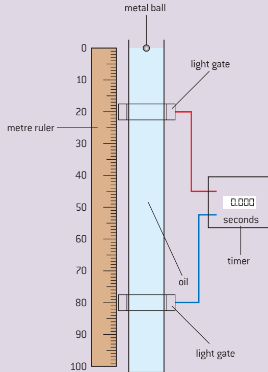
▲ Figure 13 Stokes' law investigation.
