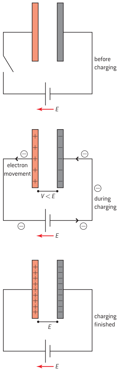
▲ Figure 1 Charging a capacitor.
