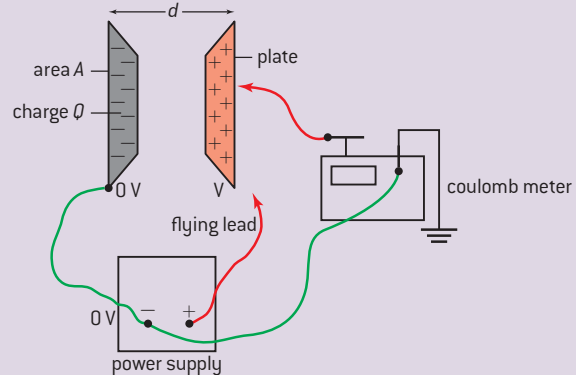
▲ Figure 1 How the charge stored on parallel plates varies.
