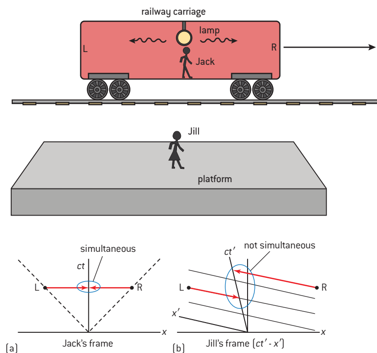
▲ Figure 4 Simultaneity at work in a spacetime diagram.
