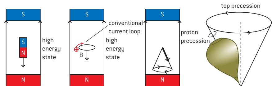
▲ Figure 8 Larmor precession.
