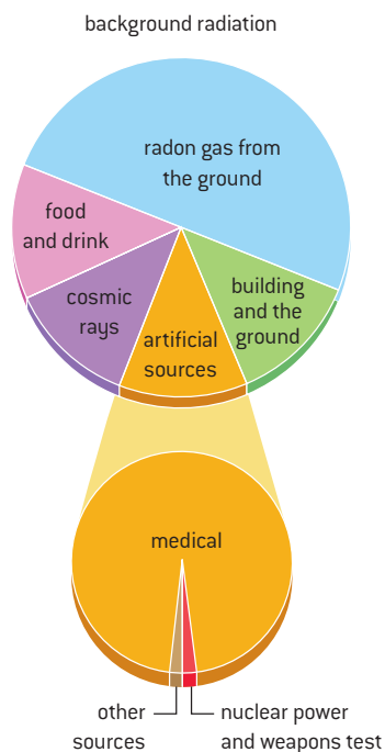
▲ Figure 12 Sources of background radiation.
