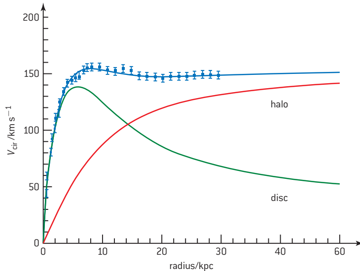
▲ Figure 8 distribution of dark matter in NGC 3198.
