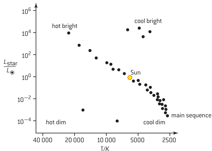
▲ Figure 6 Hertzsprung–Russell diagram.
