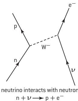
▲ Figure 5 Neutrino interacts with neutron.
