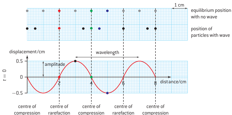
▲ Figure 7 Longitudinal wave profile.
