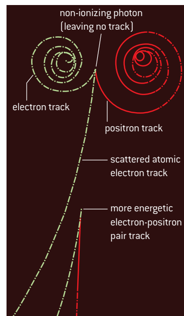
▲ Figure 5 Electron and positron tracks in a cloud chamber.
