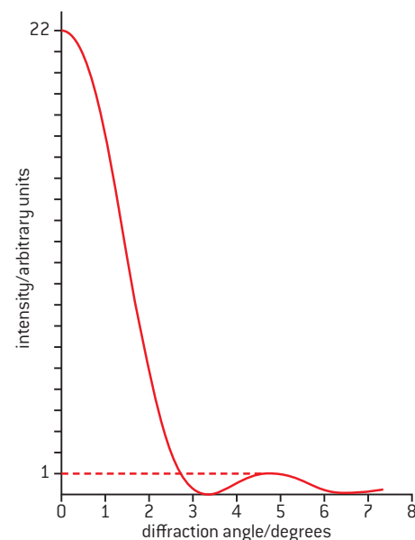
▲ Figure 9 Diffraction pattern intensity distribution.
