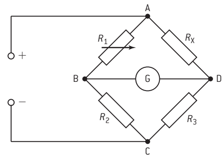
▲ Figure 12 The Wheatstone bridge.
