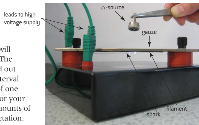
▲ Figure 11 Spark counter with alpha source.
