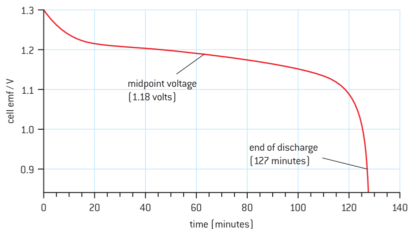
▲ Figure 3 Typical discharge–time graph for a cell.
