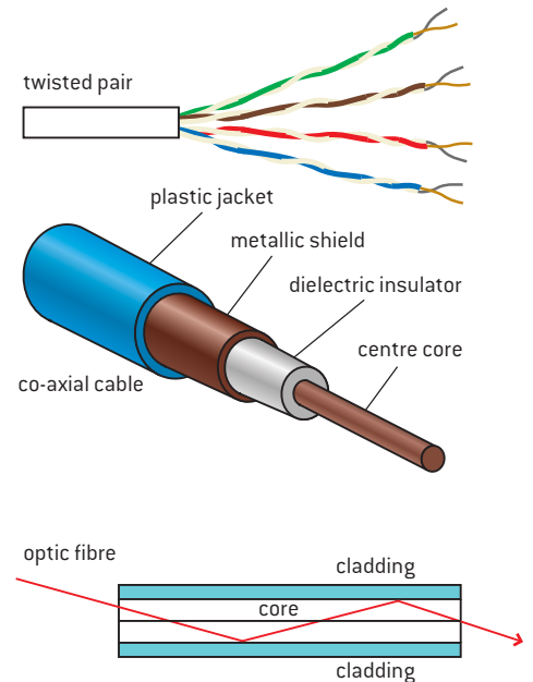
▲ Figure 2 Physical communication links.
