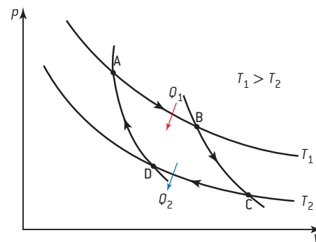
▲ Figure 10 The Carnot cycle.
