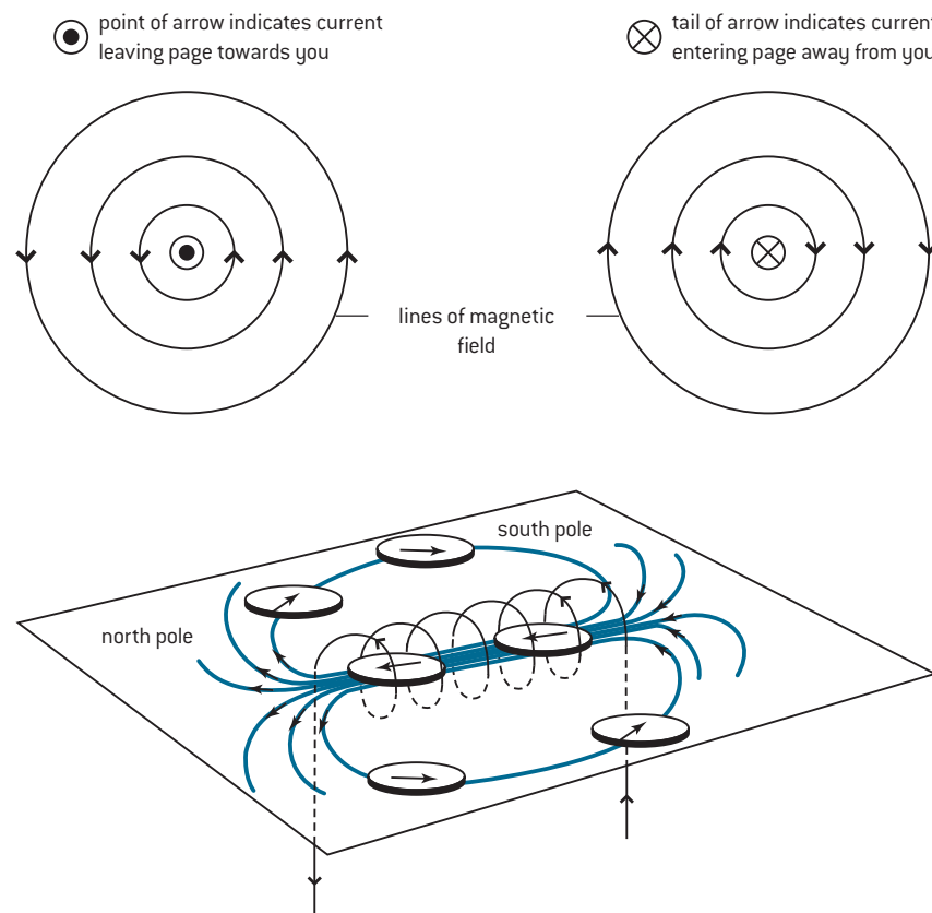
▲ Figure 3 Magnetic field patterns around current-carrying conductors.
